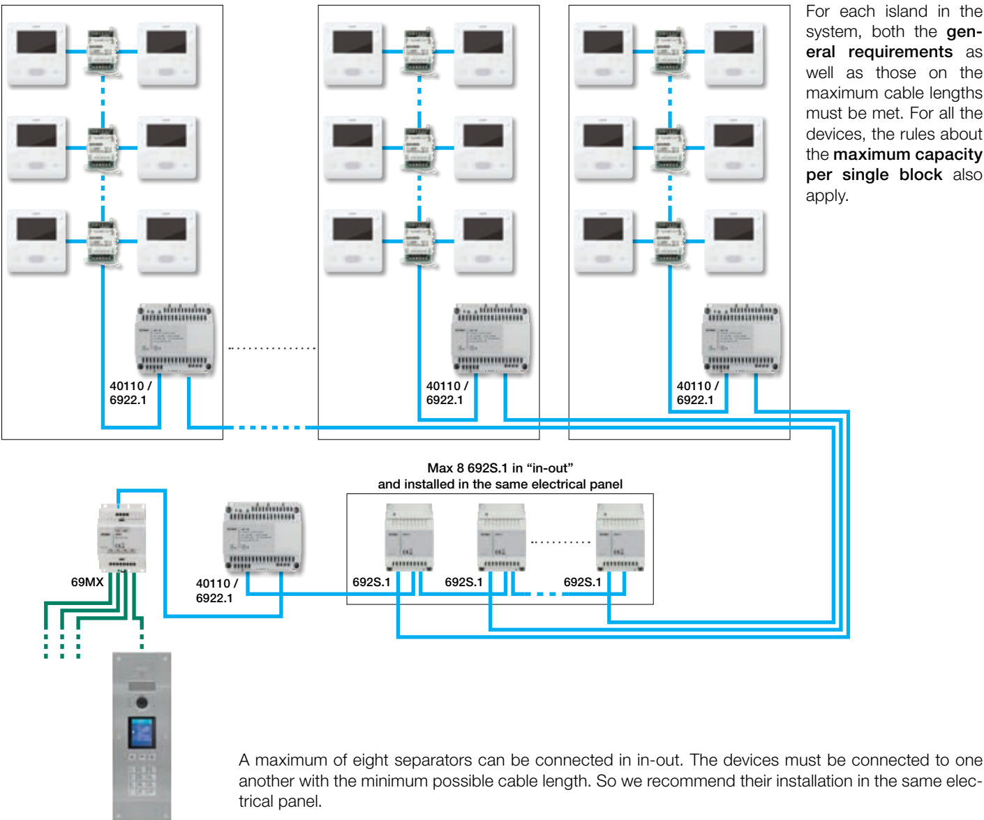
Example 1a - Separators 692S.1 connected in “in-out”.
