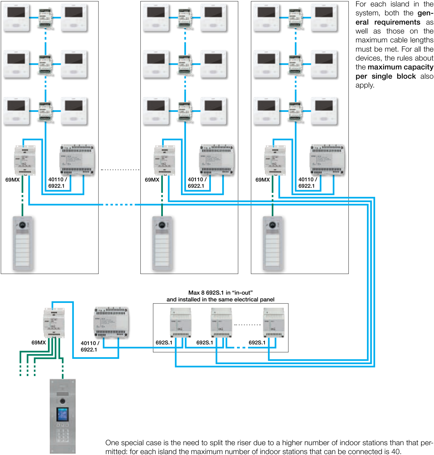
Example 1b - Separators 692S.1 connected in “in-out”.
