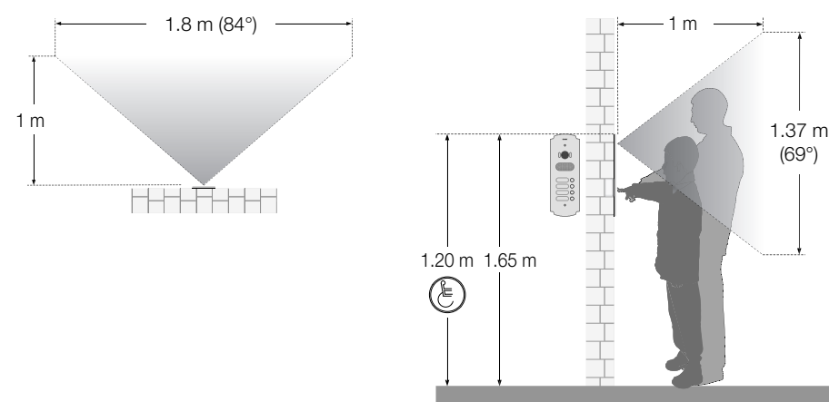
Height of installation and recording range of entrance panels
