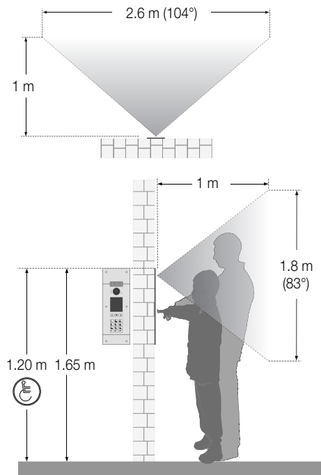
Height of installation and recording range of entrance panels
