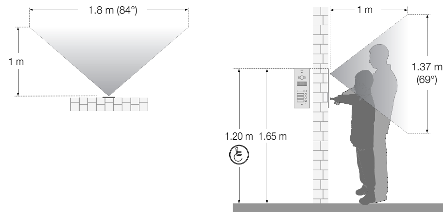
Height of installation and recording range of entrance panels
